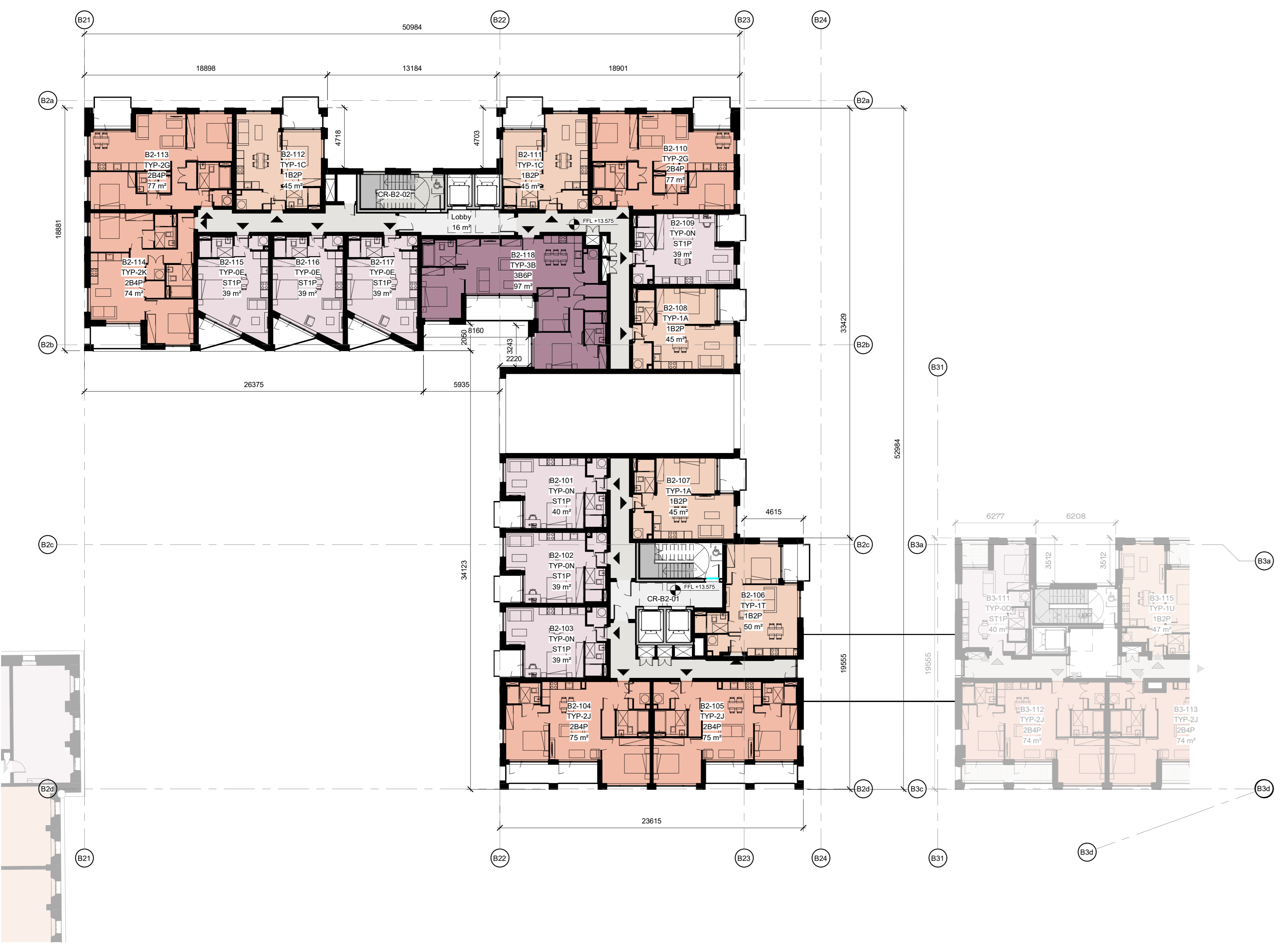
4 BLOCK B2-LEVEL 01 1:200
